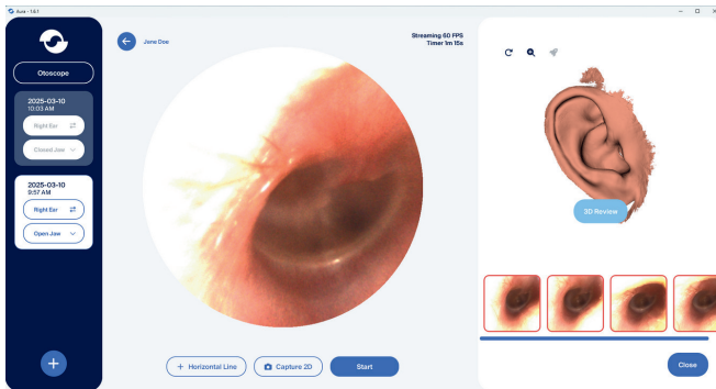
The Aurality UI – Scan window
